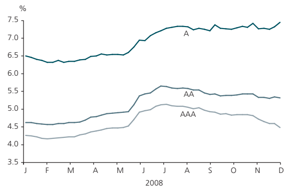
Chart 2.20 PDS Yields (5-year)
